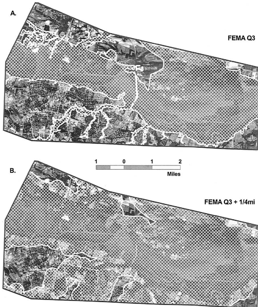
Fig. 4. Aerial photograph of flooding and floodplain representations. (a) FEMA Q3 100-year floodplain; and (b) FEMA Q3 100-year floodplain buffered 1/4 mile.
